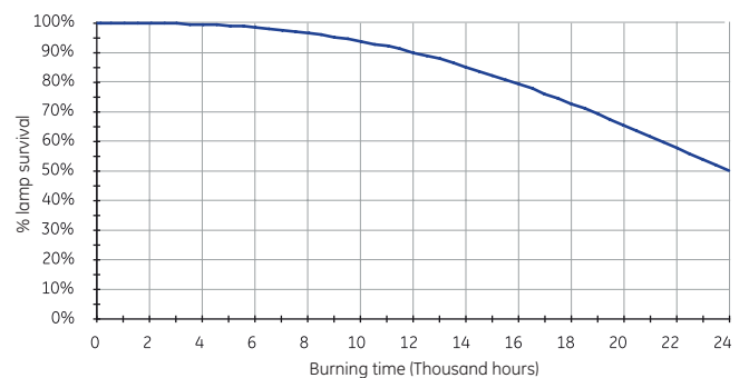
Lamp survival CMH Streetwise™ 50W EM, 70W & 100W
