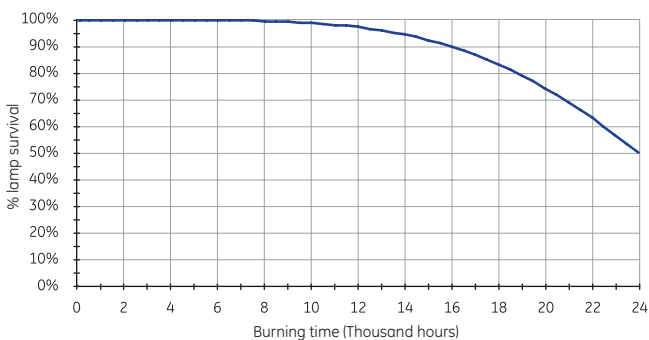
Lamp survival CMH Streetwise™ 70W & 100W Vertical burning
