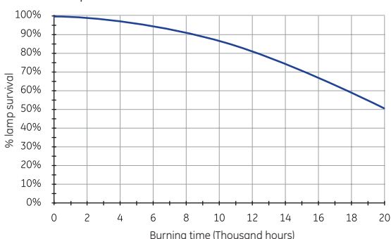
Lamp survival CMH Streetwise™ 70W & 100W Vertical burning
